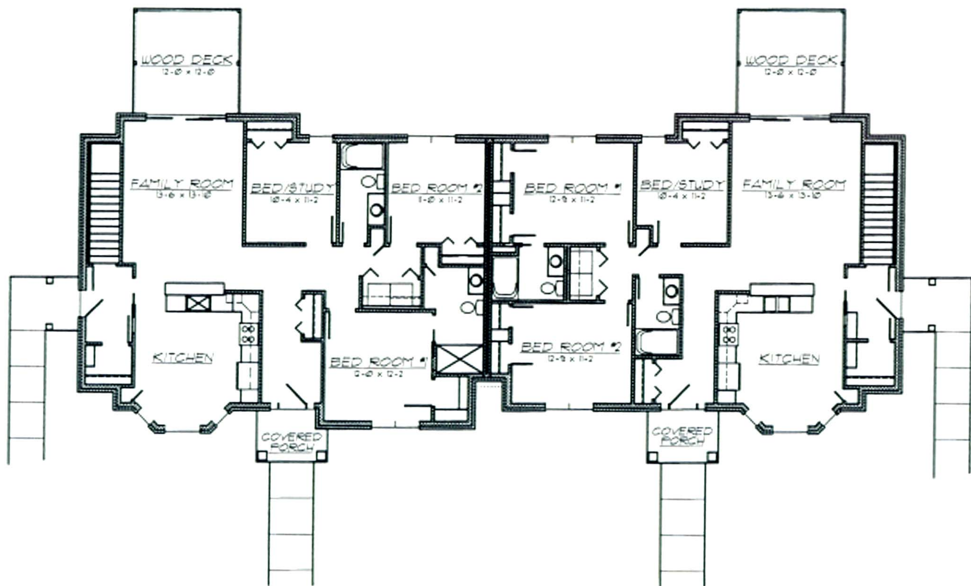
FLOOR PLAN
